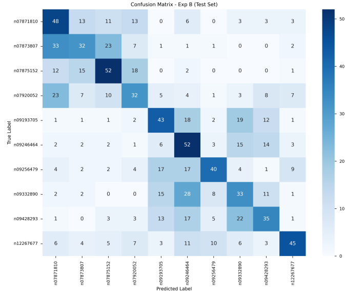
Figure 3: Confusion Matrix for Experiment B (Leaky ReLU + BN) on the Test Set.
