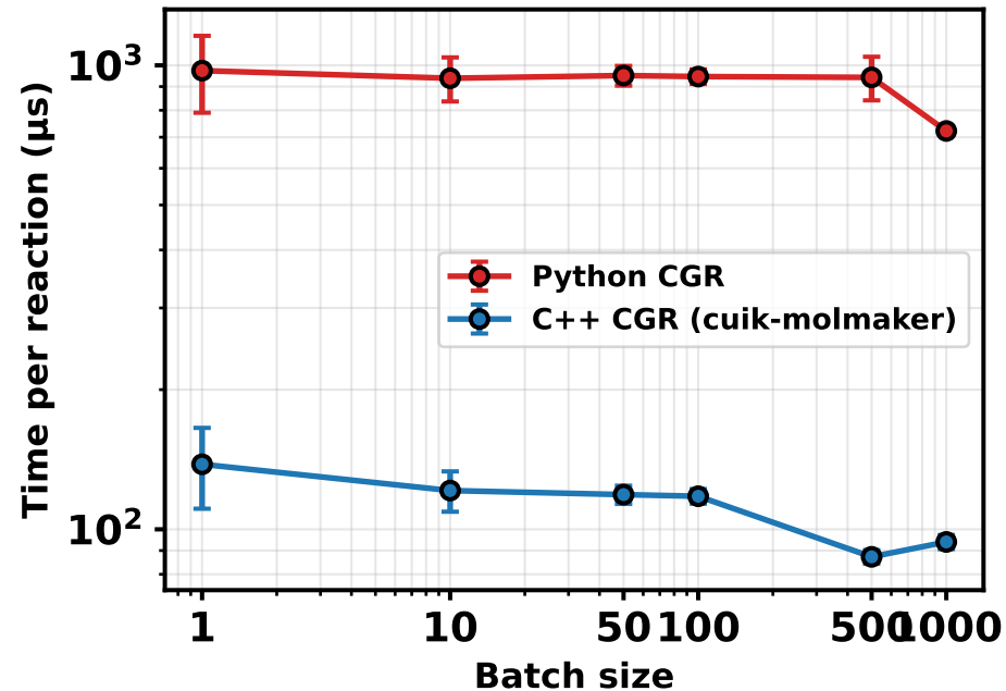
Featurization time per reaction
