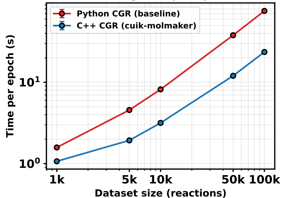
Training time per epoch
