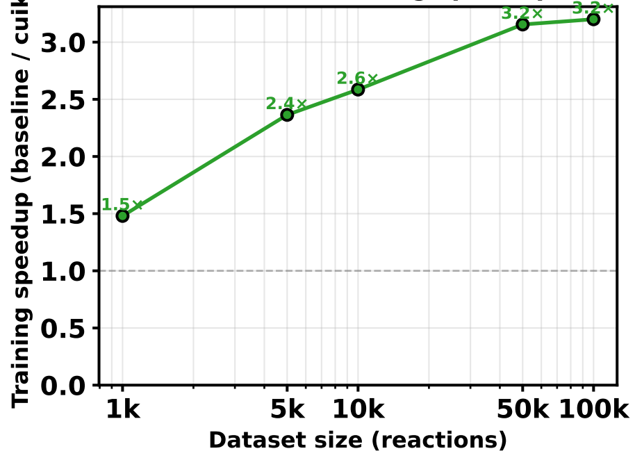
End-to-end training speedup
