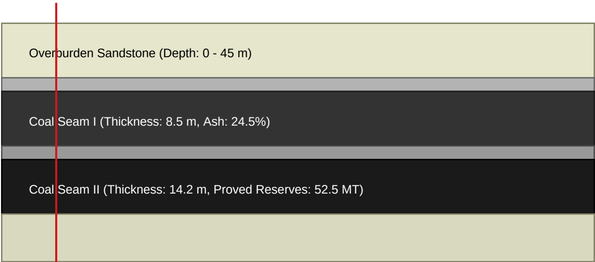
Caption: Detailed borehole litholog indicating parting and seam thicknesses.
