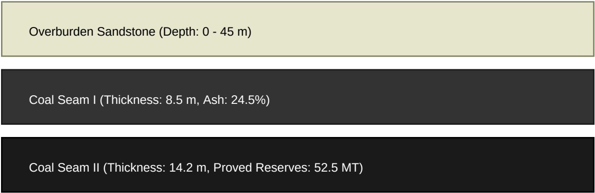
Figure 2: Stratigraphic Cross-Section of Barakar Formation at Block-IV
