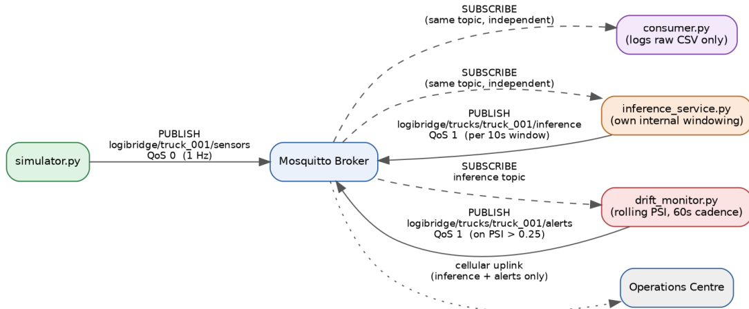
Figure 2: MQTT topic tree, QoS levels, and independent-subscriber pattern.
