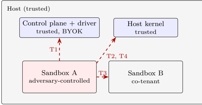
Fig. 1. Trust boundary. Adversary-controlled code executes inside a sandbox; the control plane, driver, and host kernel are trusted. Dashed arrows are the four threat classes the substrate must resist. Side channels between co-tenants on shared hardware are out of scope.
