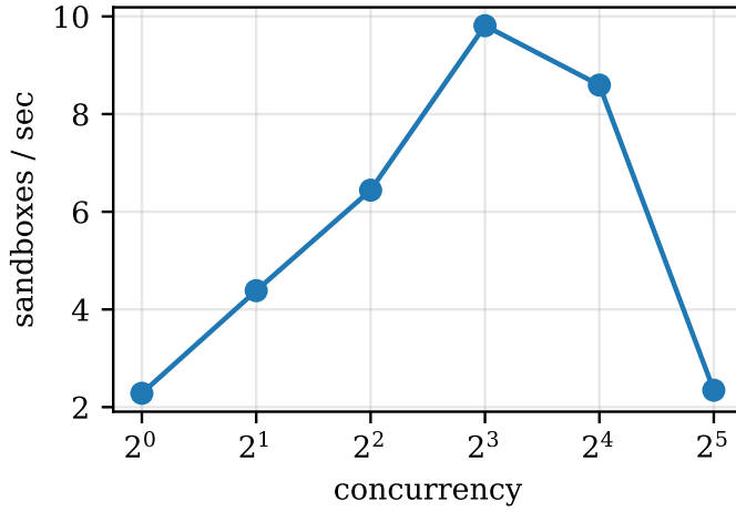
Fig. 5. Sustained sandbox-creation rate as a function of client concurrency.
