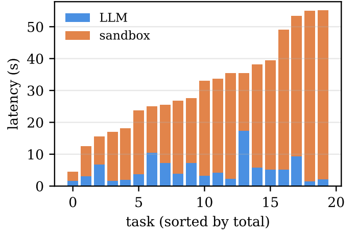
Fig. 7. Per-task LLM time versus sandbox time over 20 HumanEval-style code-generation tasks.
