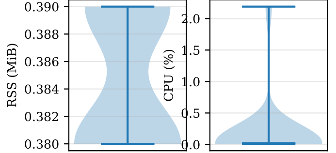
Fig. 6. Idle resident-set size and CPU per sandbox.
