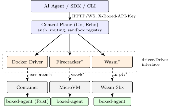
Fig. 2. Boxed architecture. The control plane drives a single narrow Driver interface, behind which the Docker driver ships today and Firecracker/Wasm drivers are stubbed. A common Rust agent runs inside every sandbox and speaks JSON-RPC over whatever byte stream the driver supplies. *Stubbed; not production-ready in the current release.
