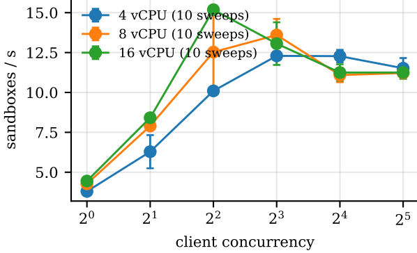
Fig. 5. Sandbox creation rate against client concurrency on 4, 8, and 16 vCPU hosts (native Linux, runc, 10 sweeps each, mean with 95% CI).
