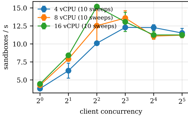
Fig. 3. Sandbox creation rate against client concurrency on 4, 8, and 16 vCPU hosts (native Linux, runc, 10 sweeps each, mean with 95% CI).
