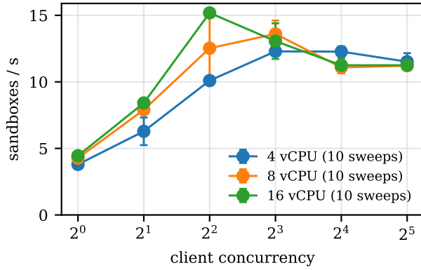
Fig. 2. Sandbox creation rate against client concurrency on 4, 8, and 16 vCPU hosts (native Linux, runc, 10 sweeps each, mean with 95% CI).
