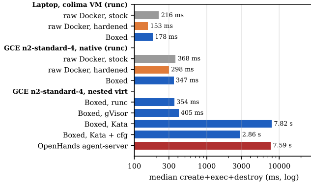
Fig. 2. Median create→exec→destroy for every configuration measured, grouped by host. Same image and command throughout; Sections VI-B, VI-G, VI-H, and VI-I give the sample sizes and confidence intervals.
