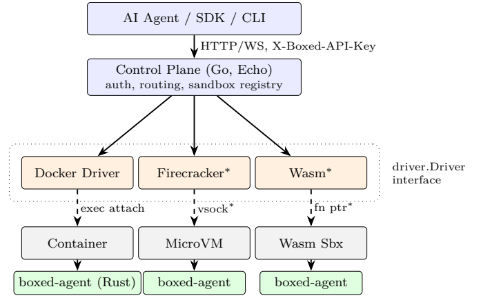
Fig. 1. Boxed architecture. The control plane drives one Driver interface. The Docker driver is the only implementation; the Firecracker and Wasm boxes show where a microVM or Wasm backend would attach. A common Rust agent runs inside every sandbox and speaks JSON-RPC over whatever byte stream the driver supplies. *Not implemented; shown as a design target only.
