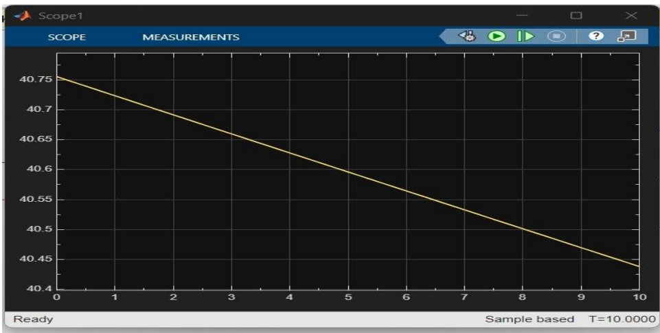
Figure 2: Pack terminal voltage declines smoothly from \sim 40.75\text{ V} to \sim 40.45\text{ V} , consistent with normal NMC discharge profile.
