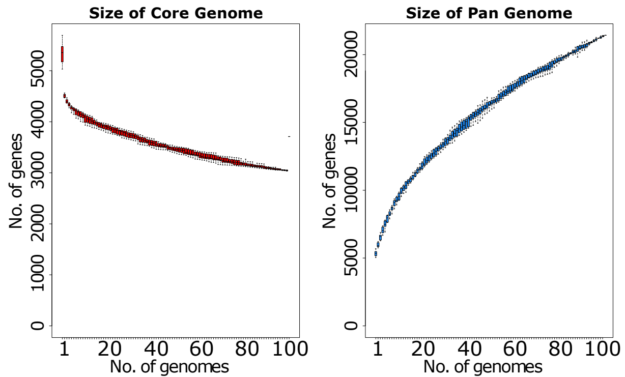
Supplementary Figure 1. Core and pan genome sizes of 100 diverse K. pneumoniae isolates. Gene rarefaction (left, core-genome) and accumulation (right, pan genome) curves are provided with the number of genes (y-axis) as a function of the number of genomes (x-axis). Core genome is defined as the number of genes found in 99% of the genomes. Boxplots indicate the variation in the number of genomes used for the calculation at each position.
