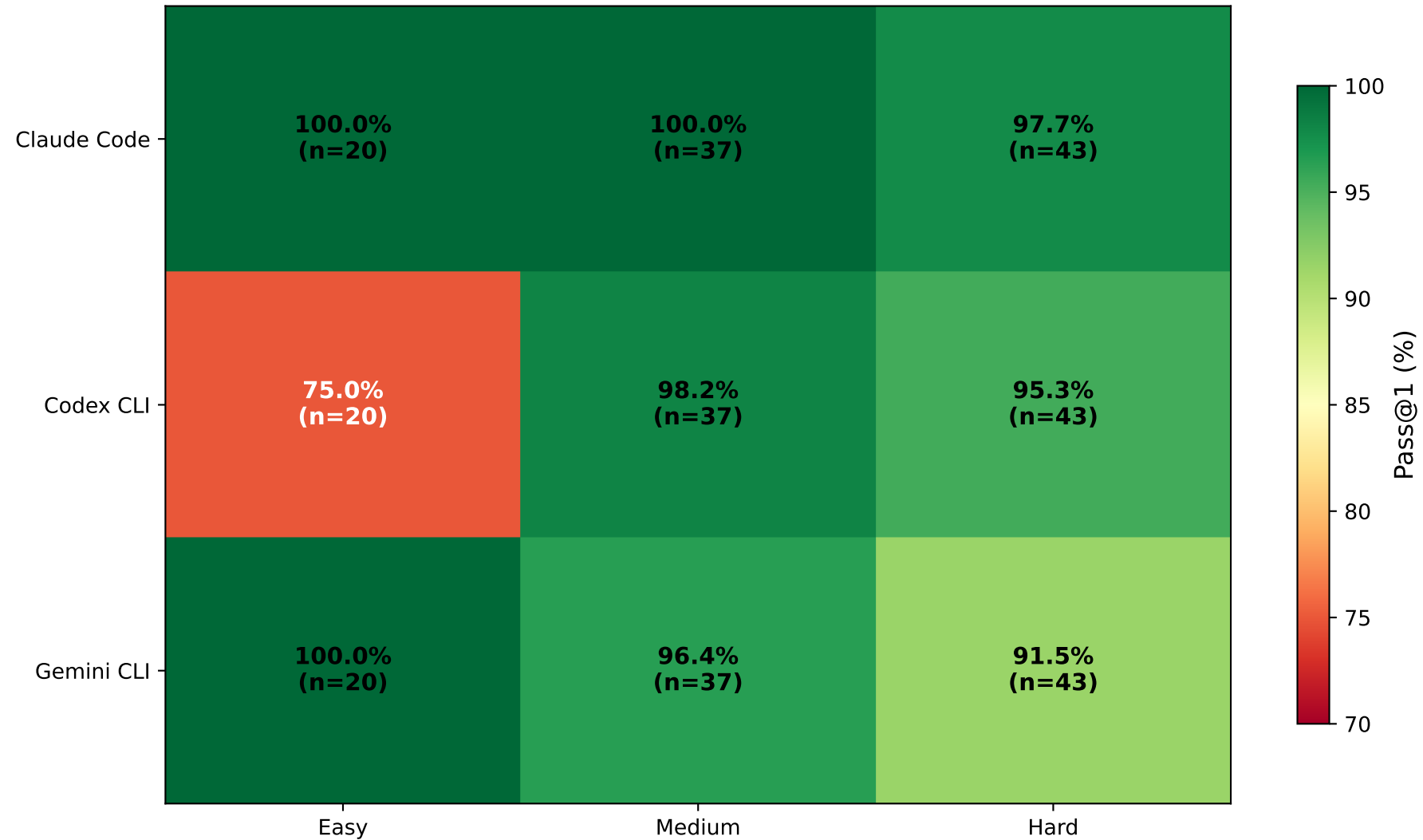
Pass@1 Rate by Task Difficulty
