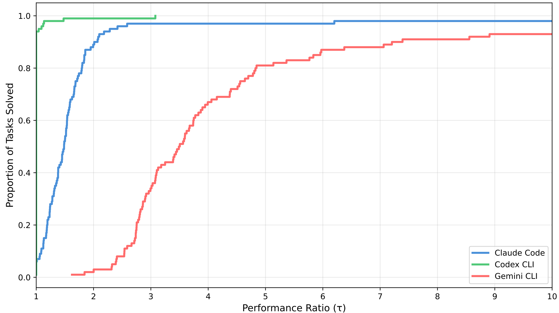
Performance Profile (Lower = Better)
