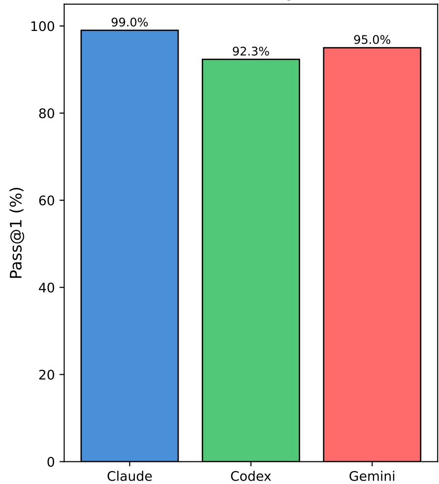
Accuracy
