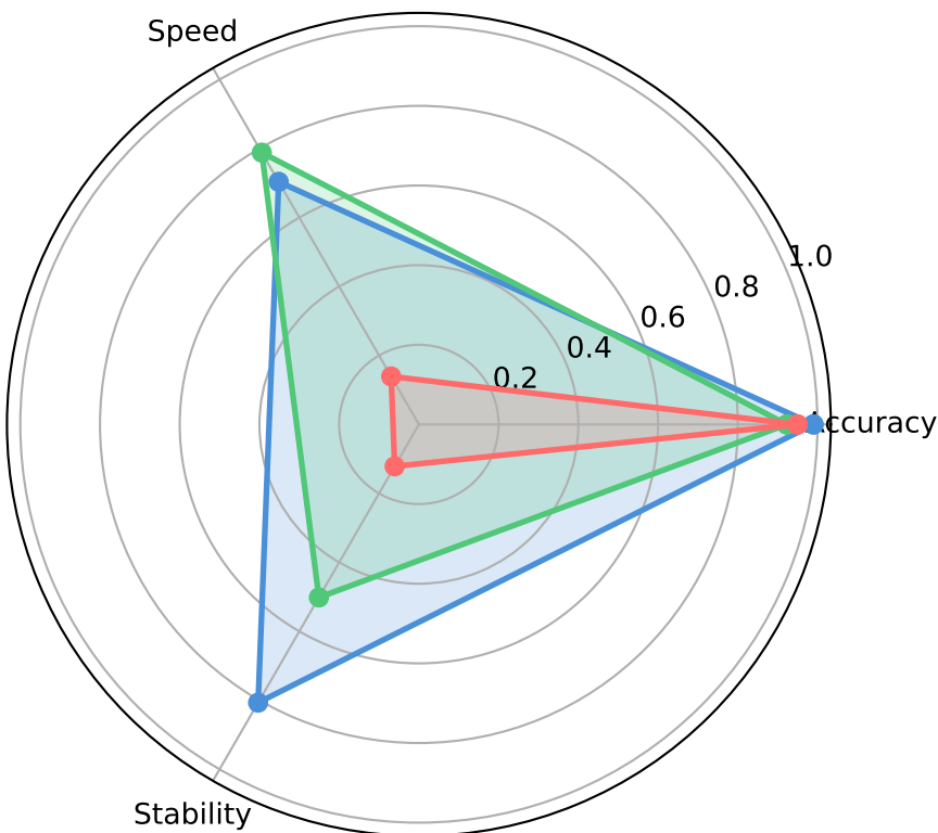
Trade-off Overview
