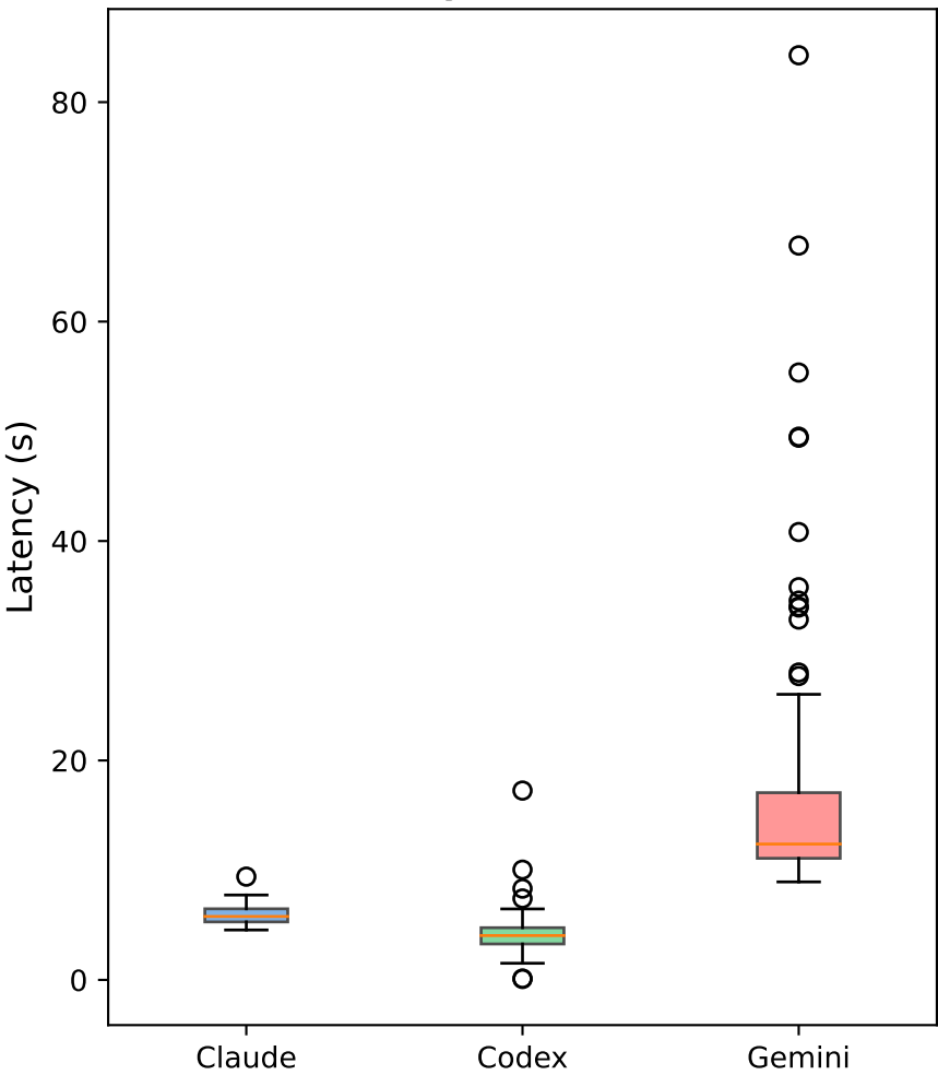
Latency Distribution
