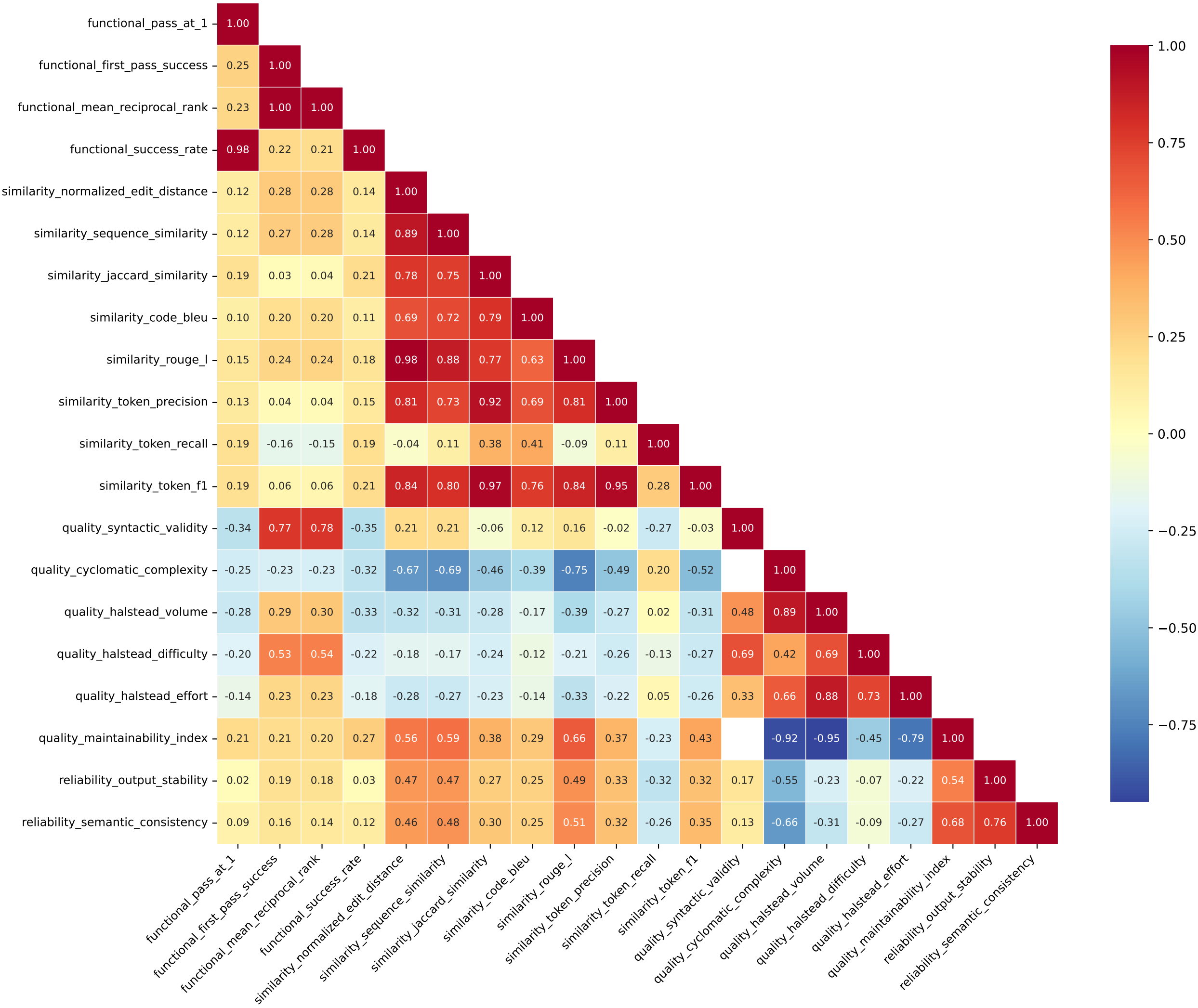
Metric Correlation Matrix
