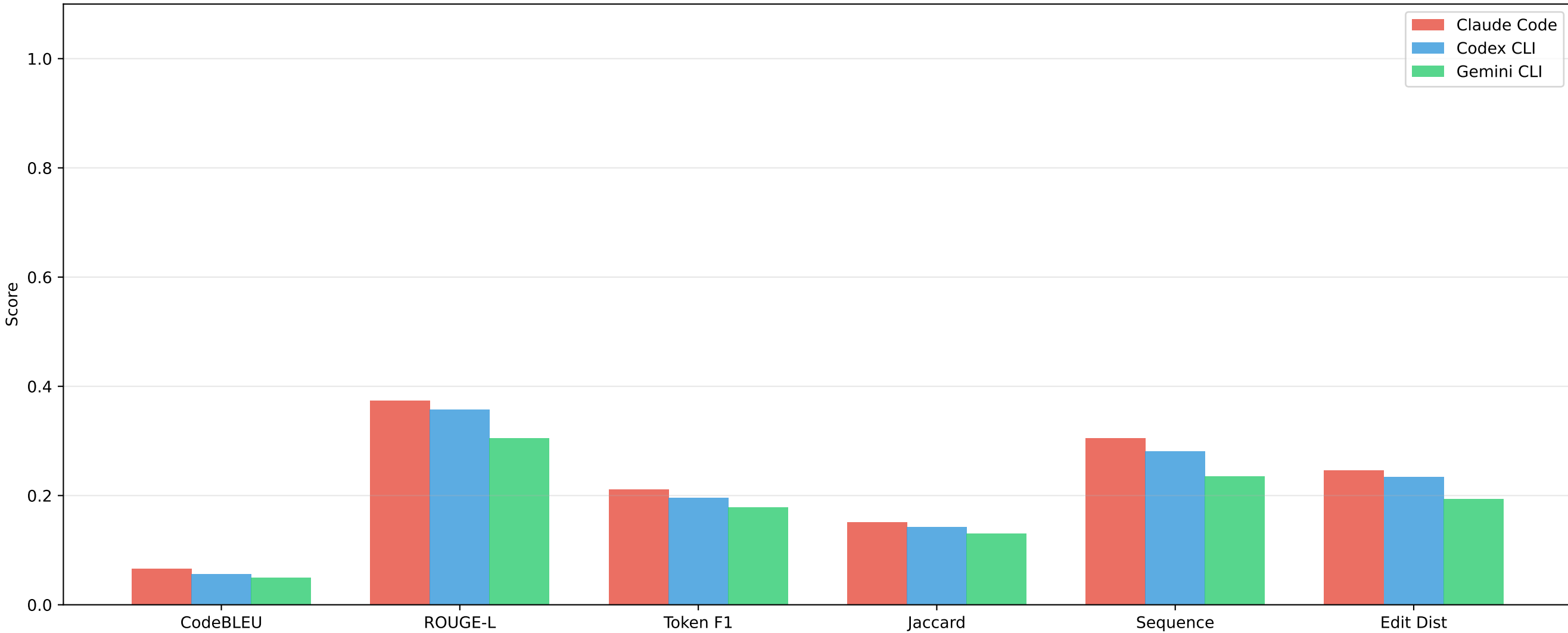
Code Similarity Metrics Comparison
