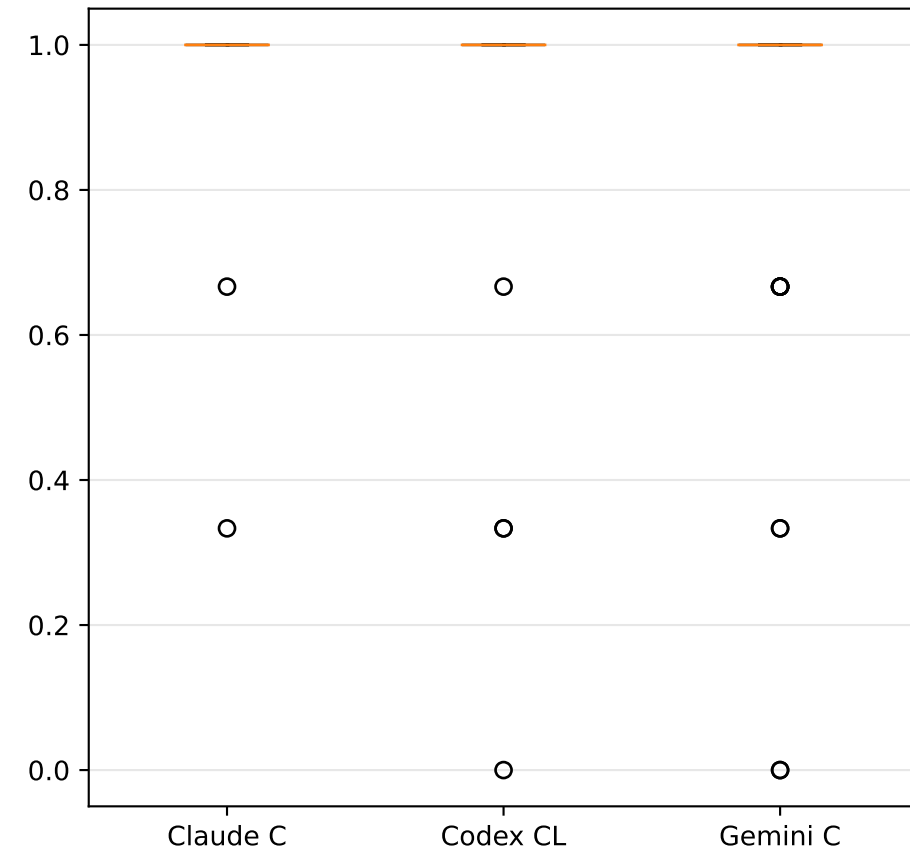
Maintainability
