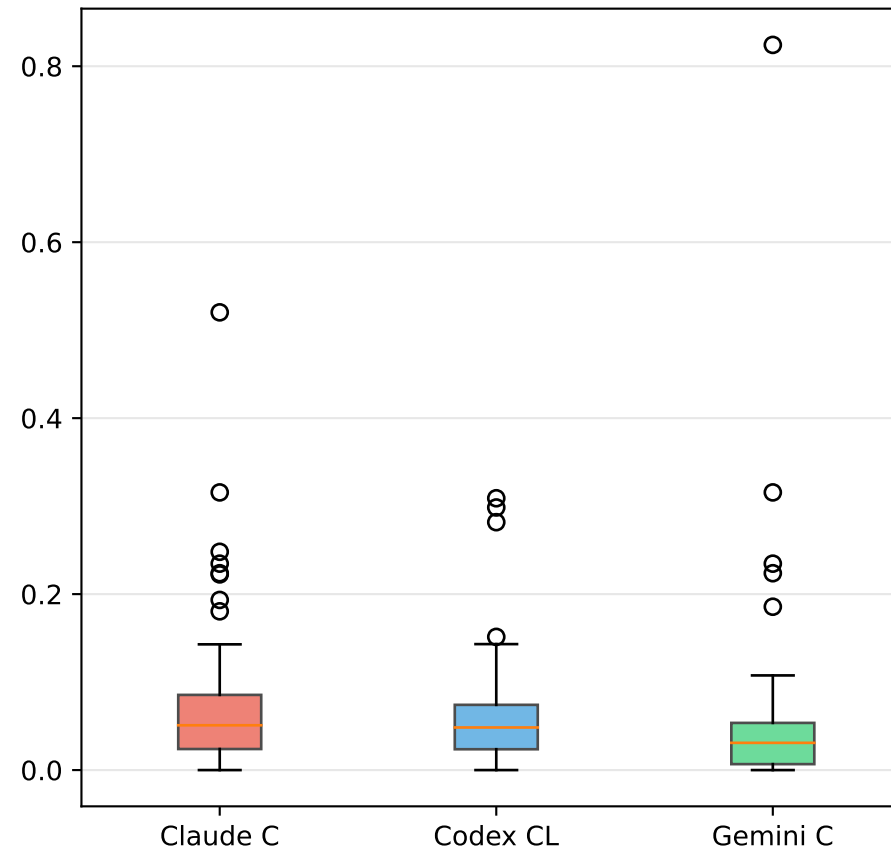
Stability
