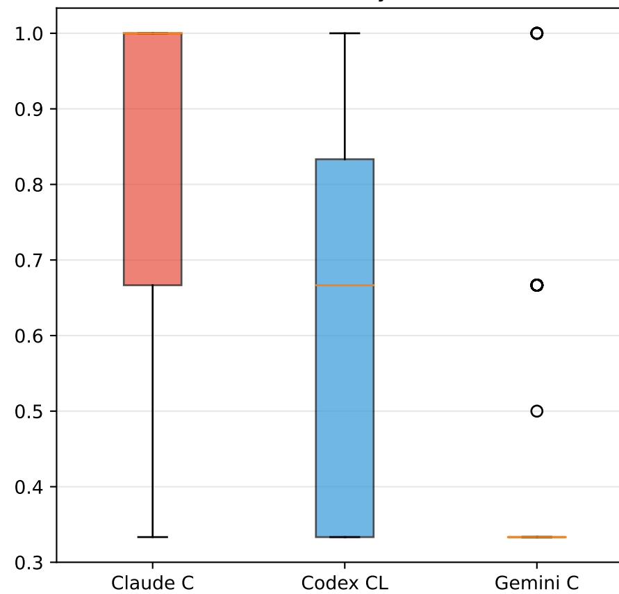
Stability
