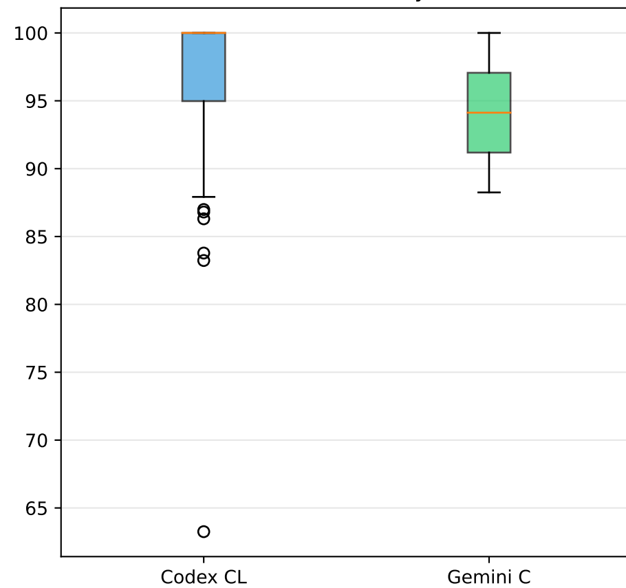
Maintainability
