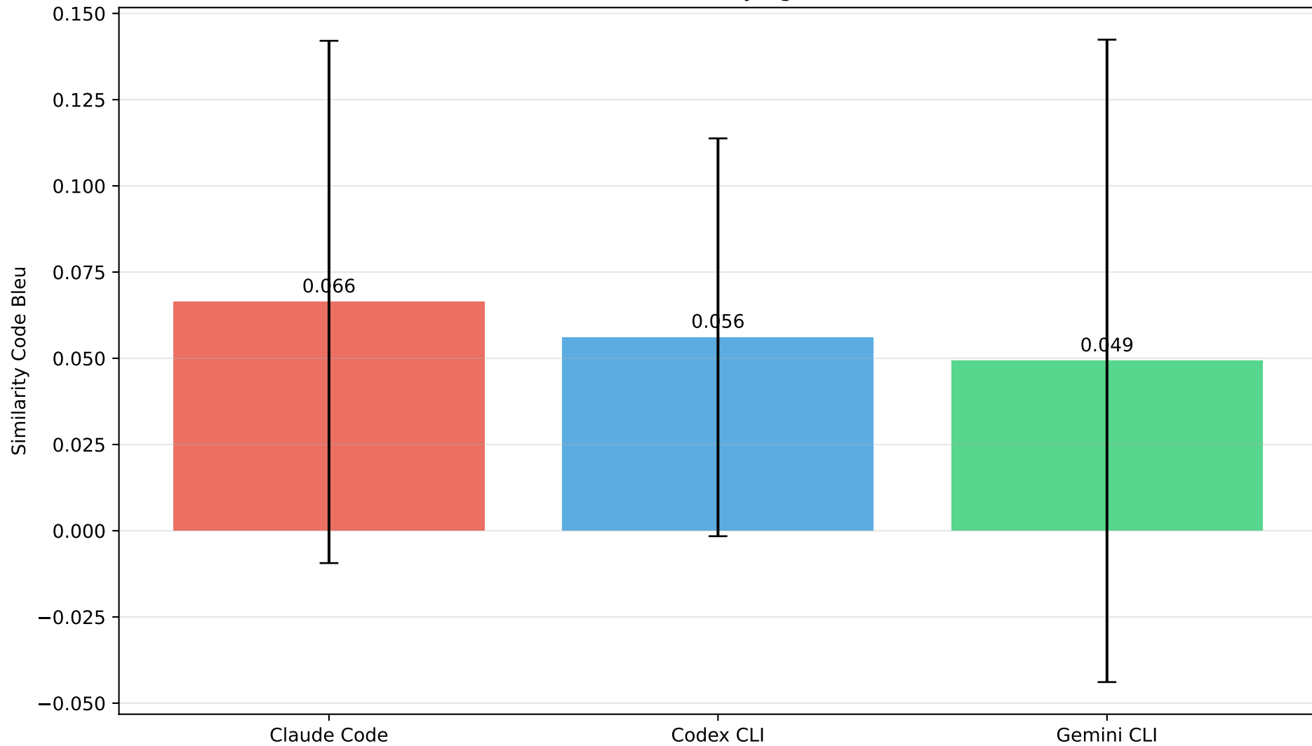
CodeBLEU by Agent
