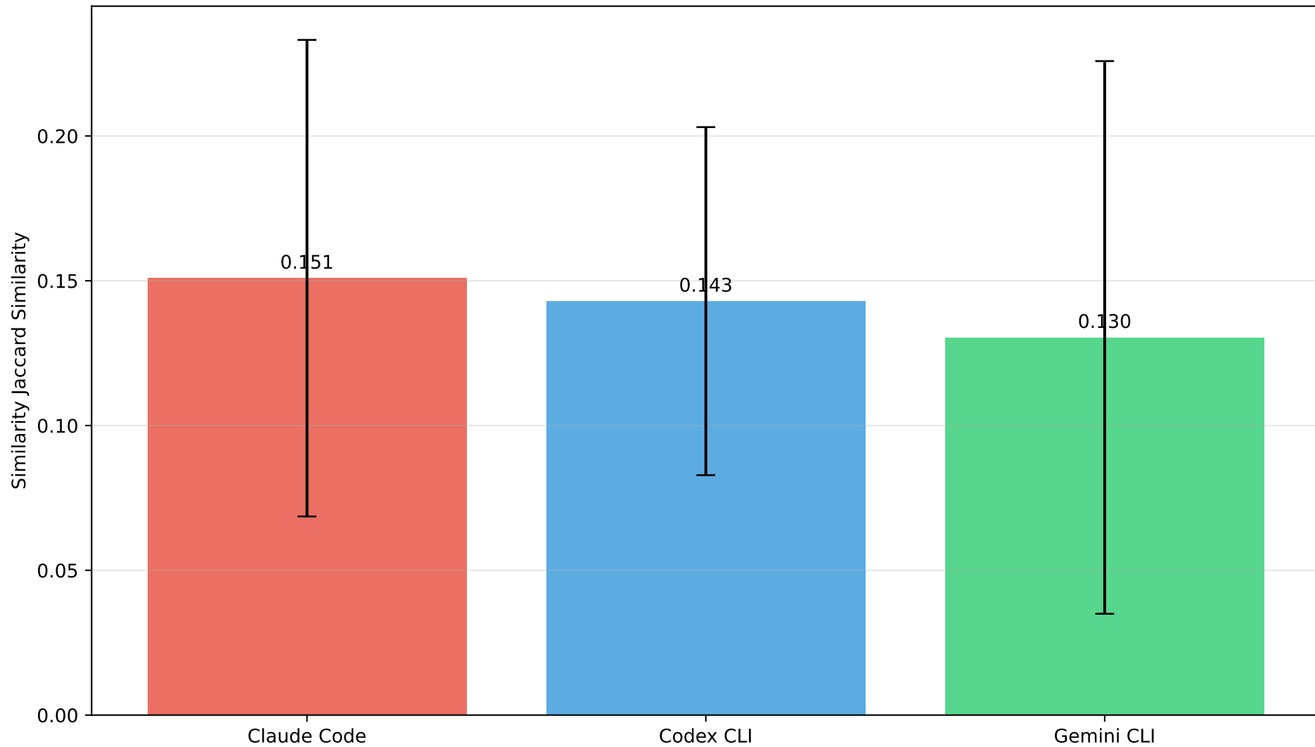
Jaccard Similarity by Agent
