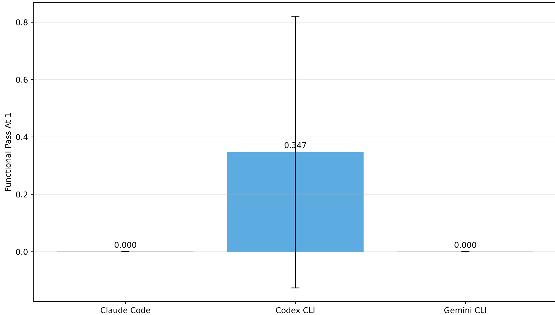
Pass@1 by Agent
