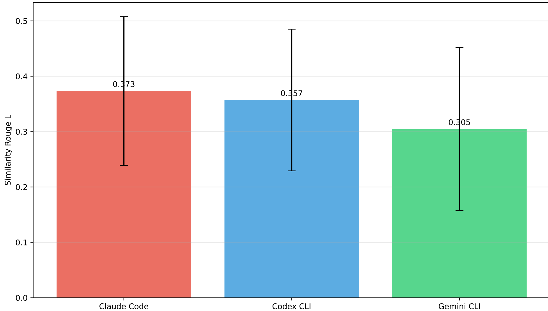
ROUGE-L by Agent
