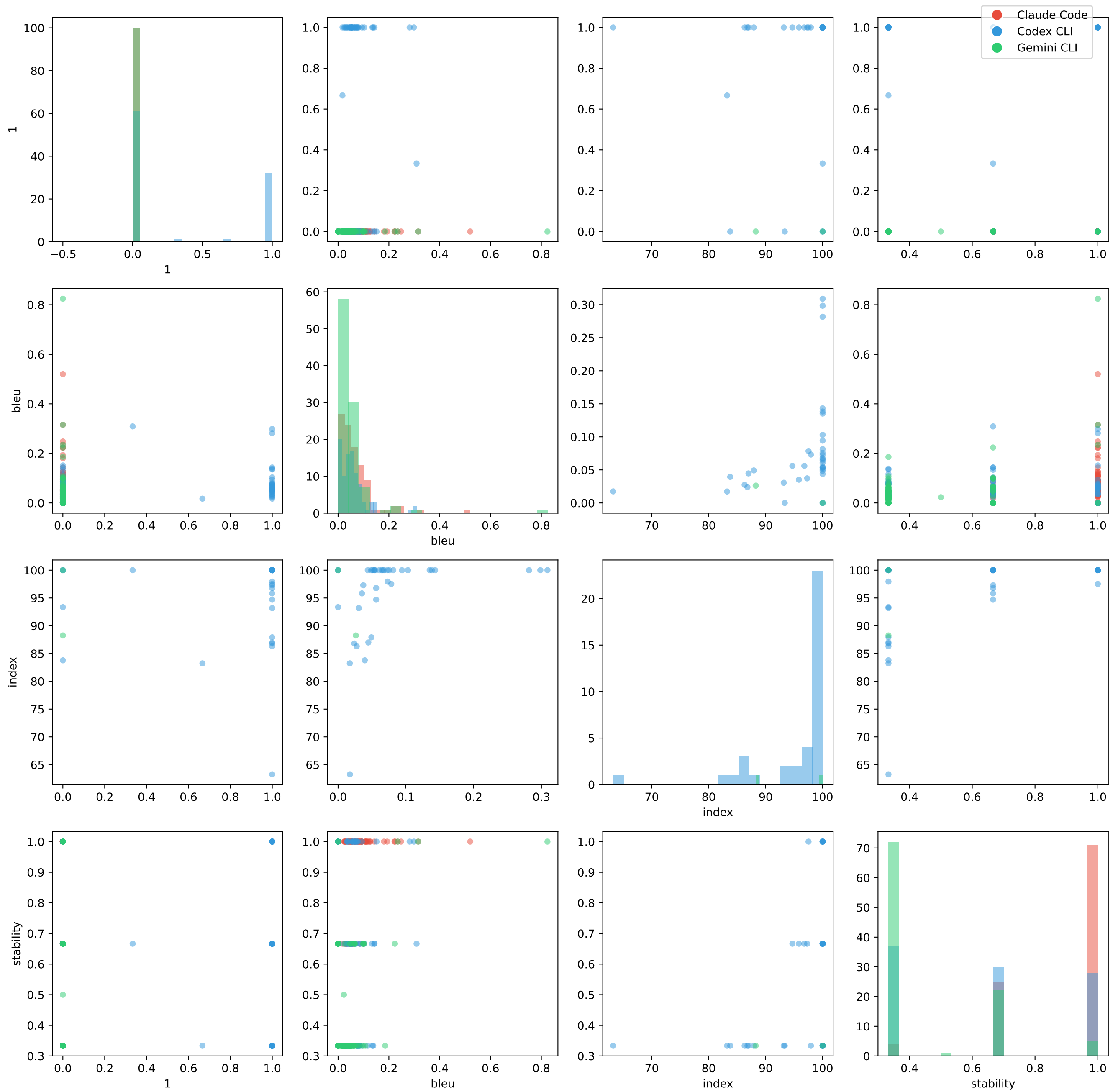
Metric Scatter Matrix
