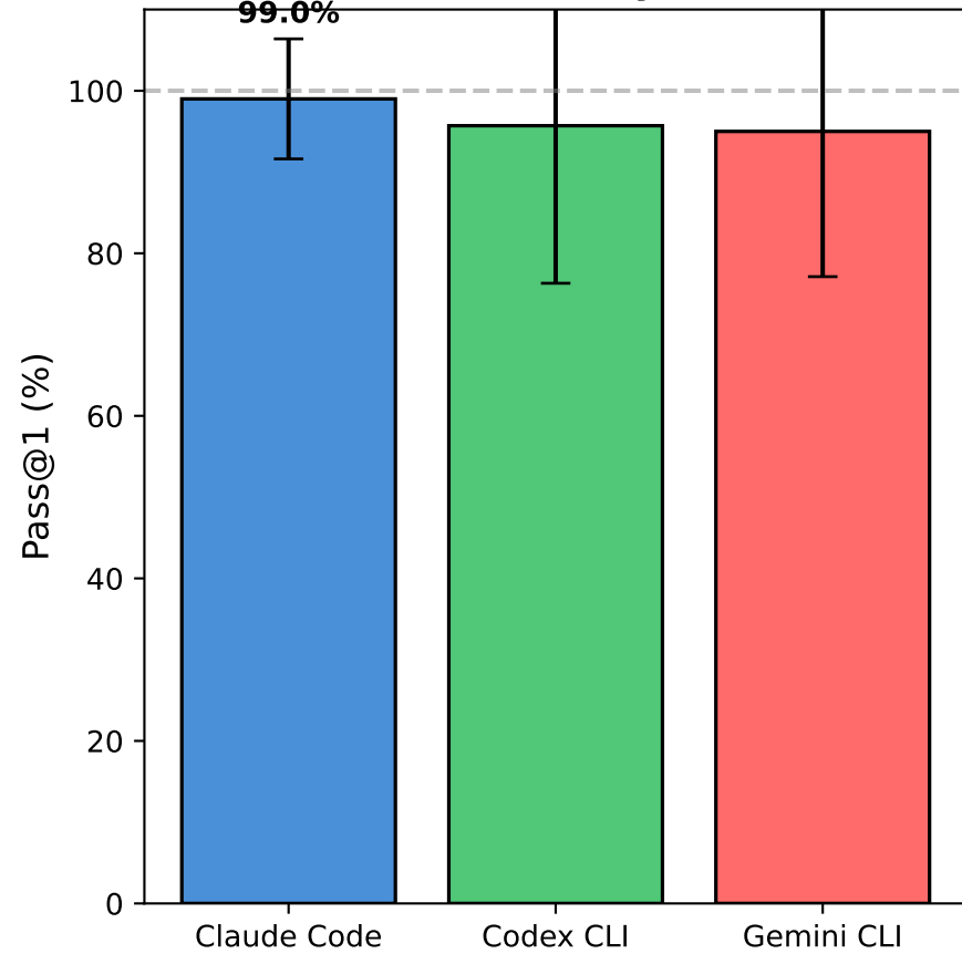
Accuracy
