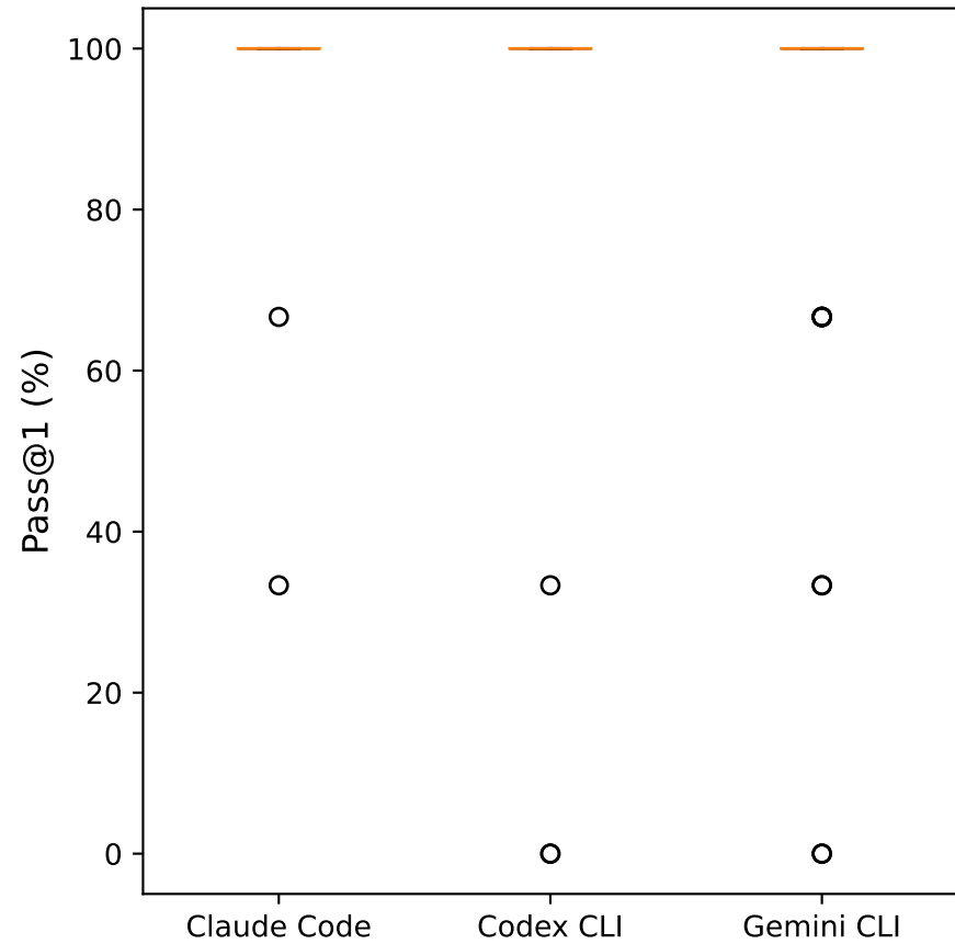
Accuracy
