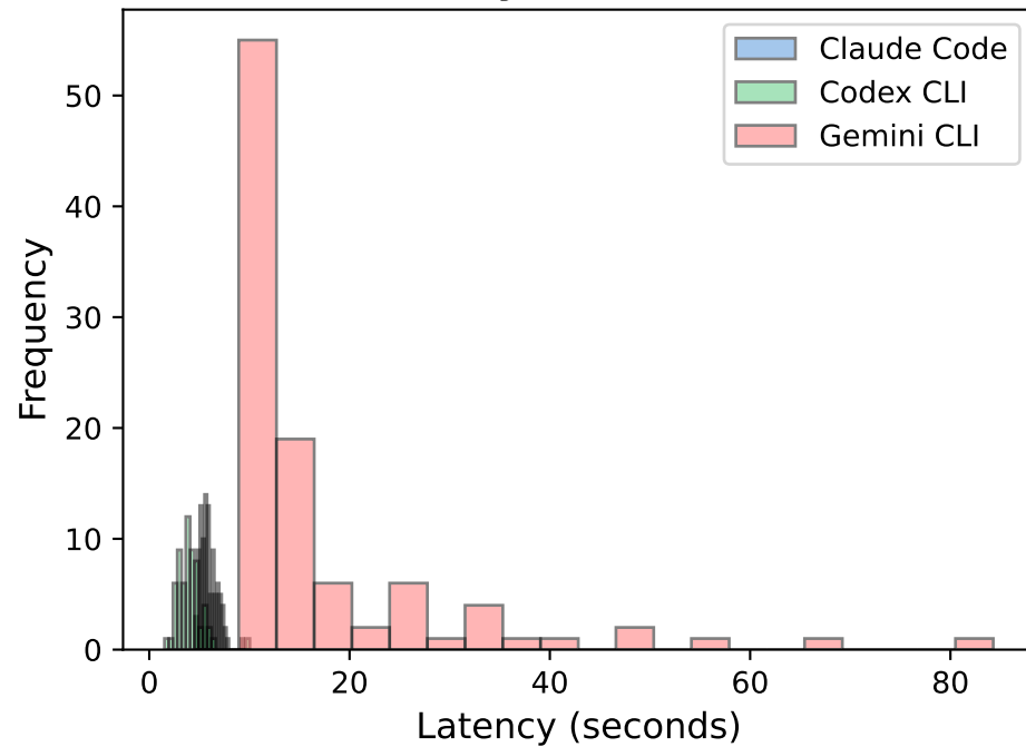
Latency Distribution
