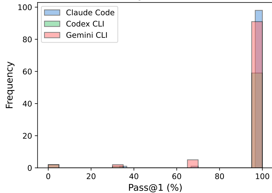
Accuracy Distribution
