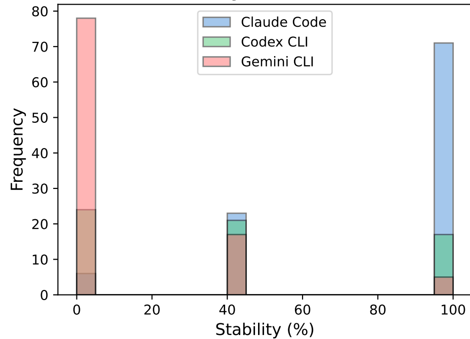
Stability Distribution
