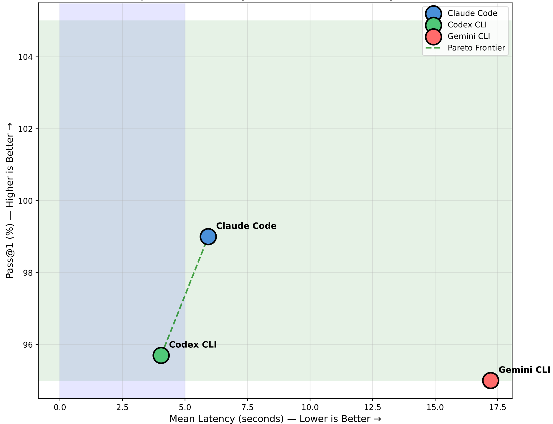
Speed vs Accuracy Trade-off (Pareto Analysis)
