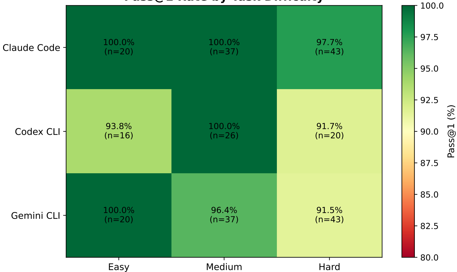
Pass@1 Rate by Task Difficulty
