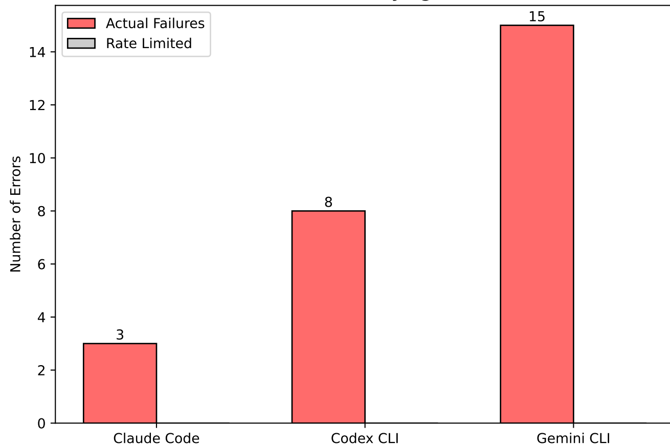
Error Count by Agent
