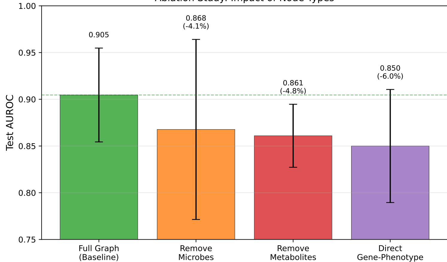
Ablation Study: Impact of Node Types
