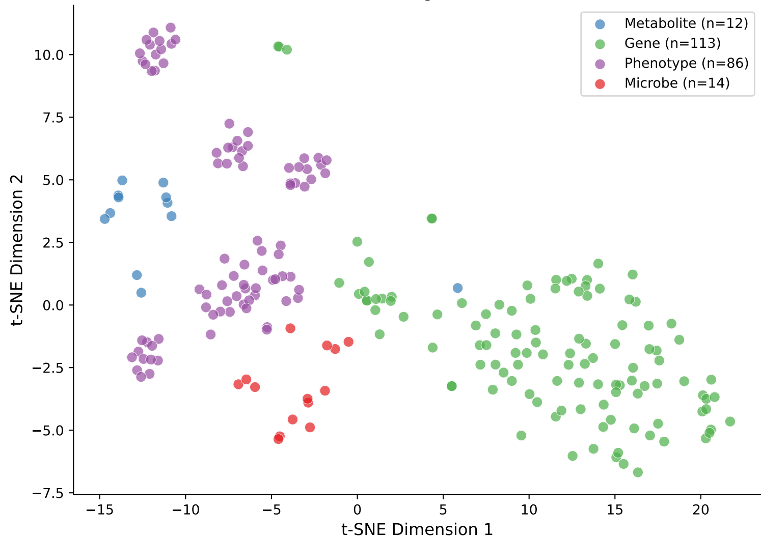
Learned Node Embeddings (t-SNE Visualization)
