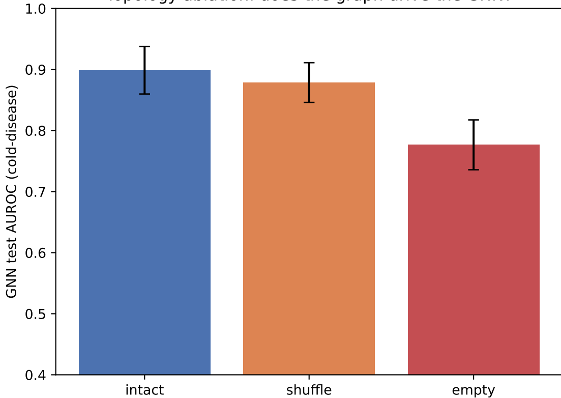
Topology ablation: does the graph drive the GNN?
