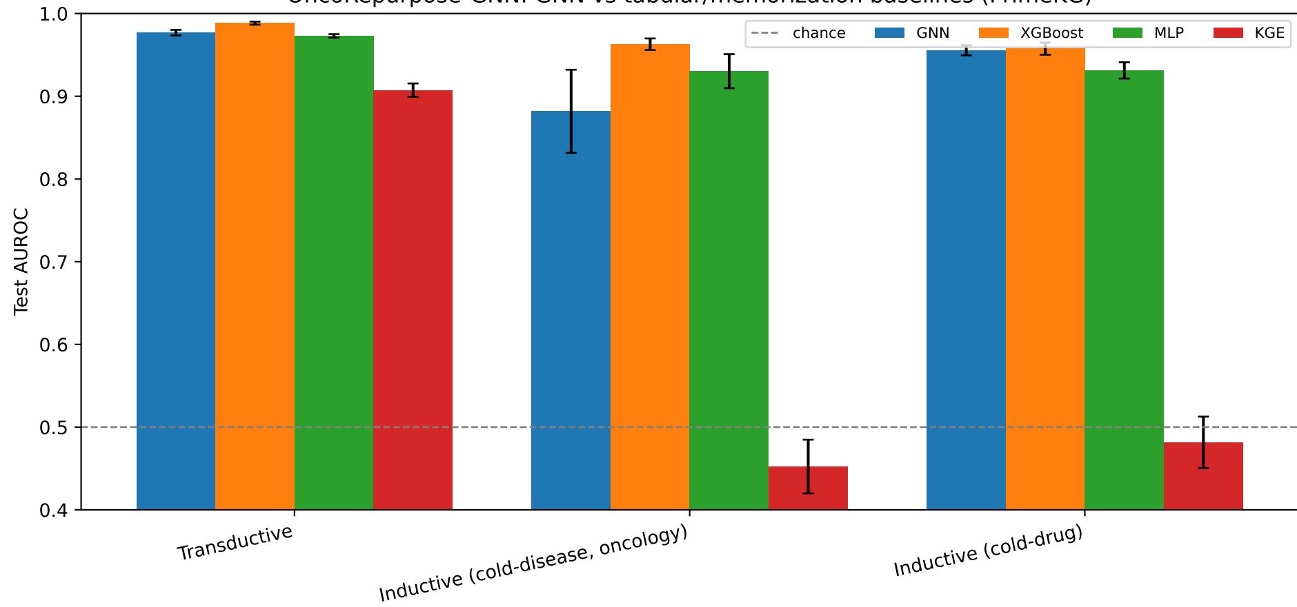
OncoRepurpose-GNN: GNN vs tabular/memorization baselines (PrimeKG)
