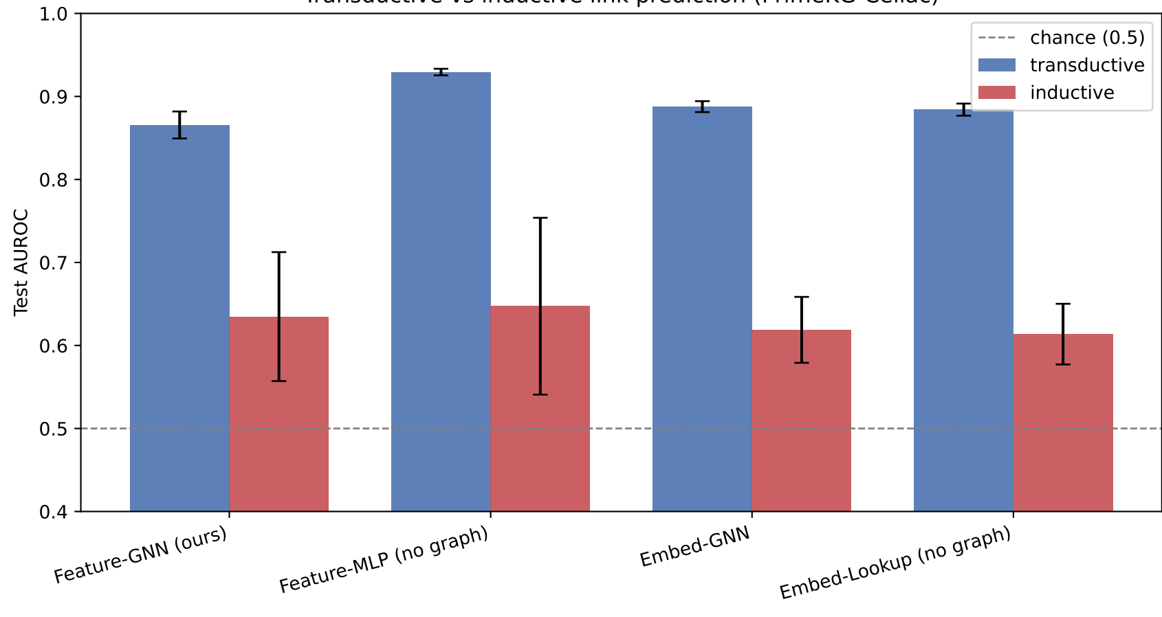
Transductive vs inductive link prediction (PrimeKG-Celiac)
