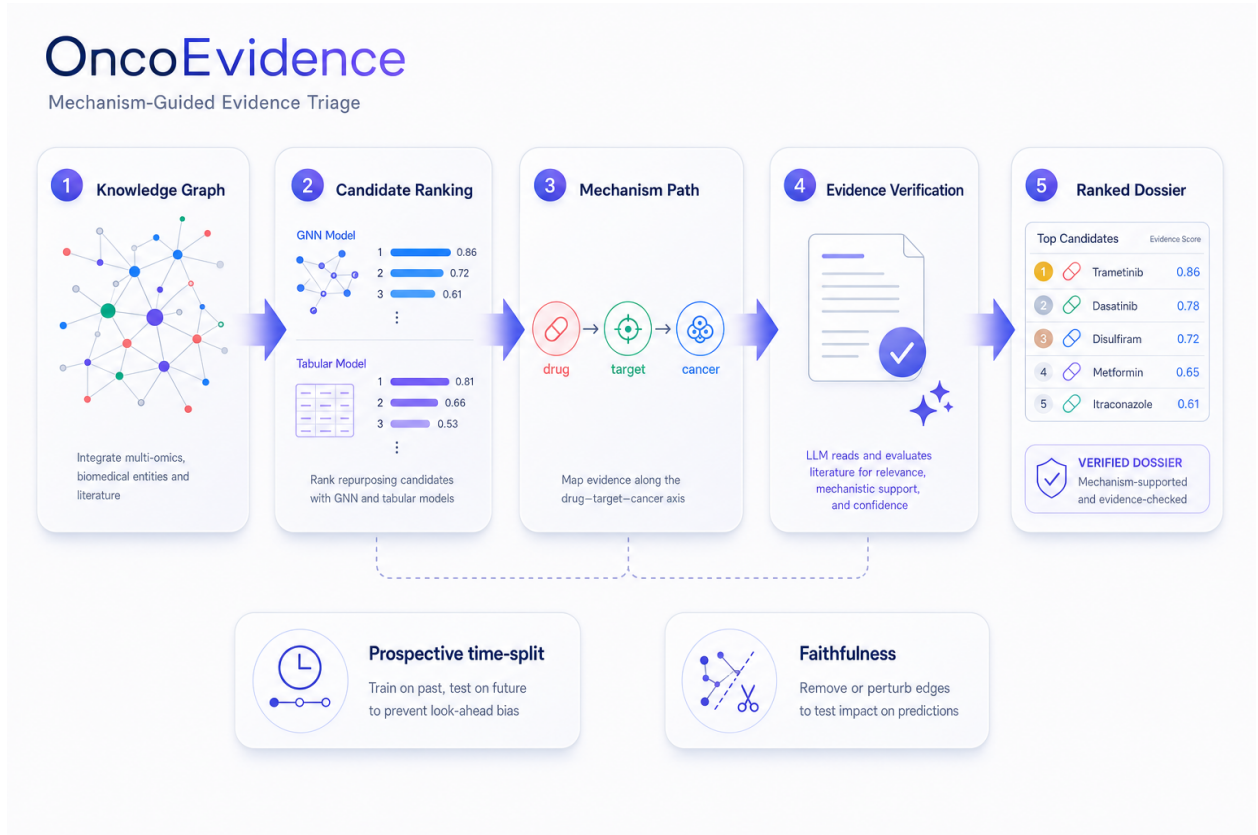
Figure 1: The OncoEvidence pipeline. We rank drug–disease candidates over PrimeKG, extract a multi-hop mechanism path (drug → target → cancer gene → cancer), verify it against Europe PMC abstracts with an LLM, and emit an evidence-backed ranked dossier. Two audits stress-test the system: a prospective time-split (train on past, test on future) and a counterfactual faithfulness test (remove mechanistic edges and re-evaluate).
