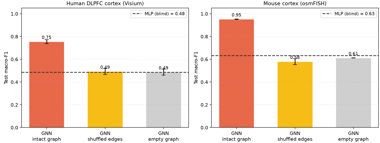
Figure 4: The same falsification test, visualized on both tissues. Only the intact spatial graph clears the MLP reference line; shuffled/empty graphs fall back to it.
