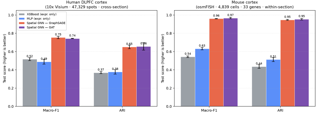
Figure 3: Headline comparison. On both human DLPFC (Visium) and mouse cortex (osmFISH), the spatial GNN (GraphSAGE / GAT) substantially outperforms XGBoost and MLP, which see the same expression features but not the tissue graph.
