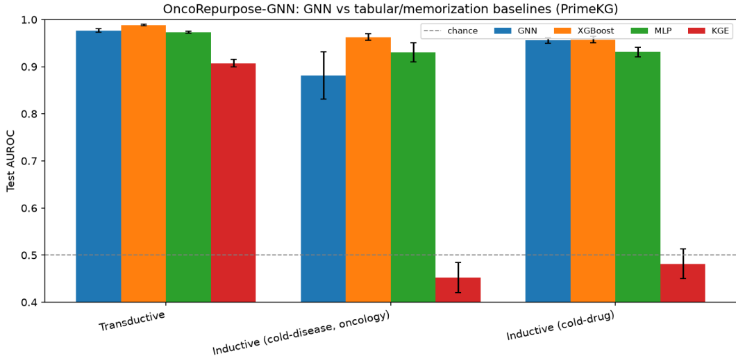
Figure 3: Benchmark AUROC by regime and model (5 seeds, error bars = std). XGBoost (or a tie) leads everywhere; KGE collapses on the inductive splits.
