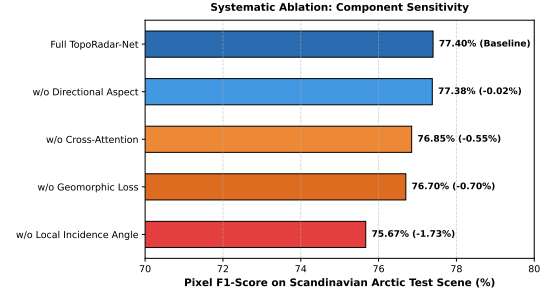
Fig. 4 Systematic component-wise ablation breakdown on the Scandinavian Arctic test scene, showing performance sensitivity to Local Incidence Angle (LIA), Aspect-Look Alignment, Radar-Topographic Cross-Attention (RTCAB), and Geomorphically Bounded Loss (Geo-Loss). The x-axis is truncated to the 70%–80% F1 dynamic range.
