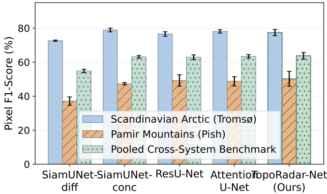
Fig. 2 Quantitative cross-system generalization performance across evaluated deep architectures on unseen mountain ranges (Scandinavian Arctic in Tromsø and Central Asian Pamir Mountains in Tajikistan), reporting Mean \pm Standard Deviation across 3 independent training seeds.
