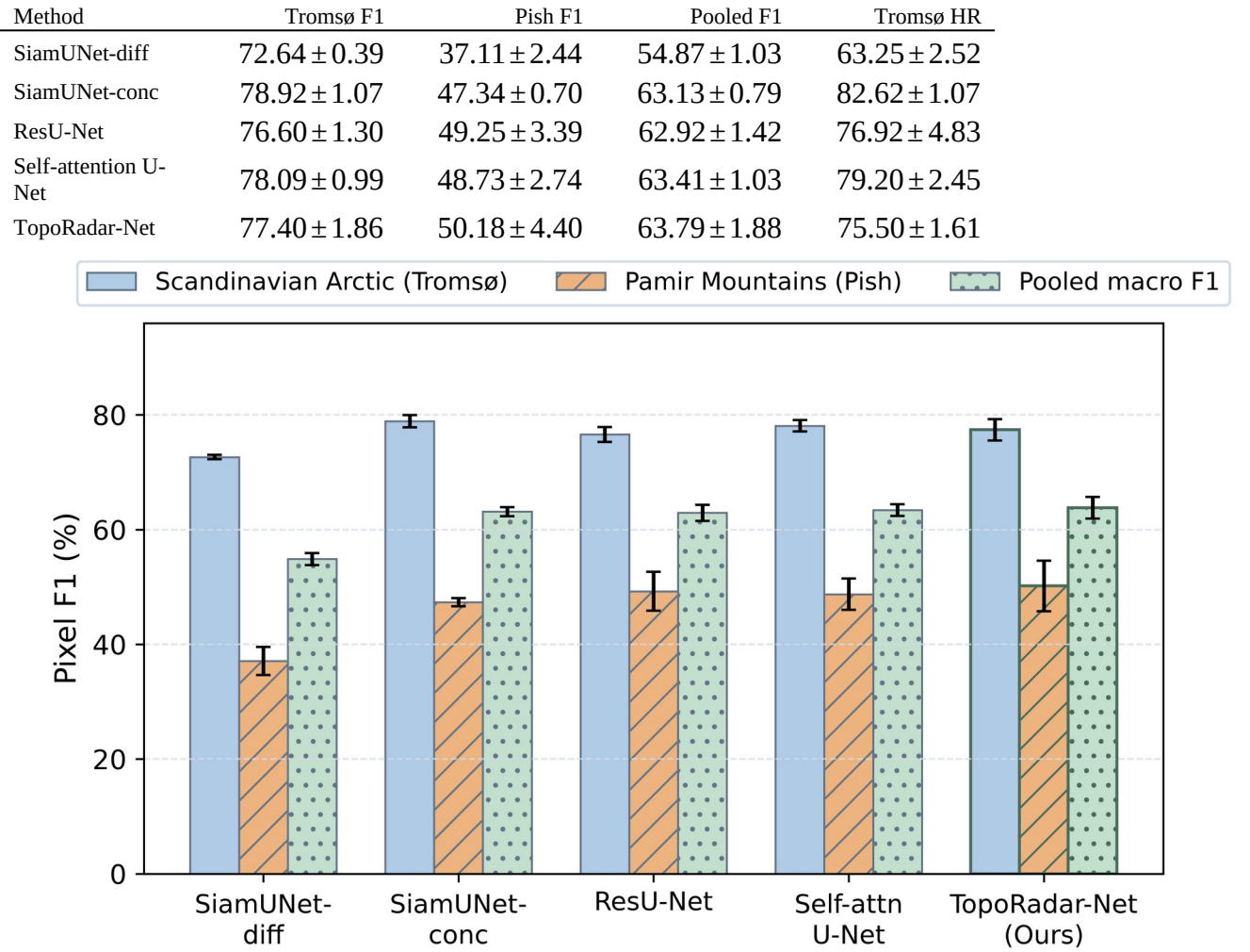
140 Fig. 2 Zero-shot pixel F1 across held-out Tromsø, Pish, and their macro average. Error bars show 141 descriptive population standard deviation over three fixed training seeds 143 The 339-block seed-42 bootstrap gives a +3.27-percentage-point micro-F1 difference from the self- 144 attention U-Net (95% CI +1.12 to +5.37, p=0.010 ), but repeating the bootstrap by training seed
