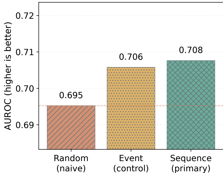
(b) AUROC difference: random – sequence = -0.0124
