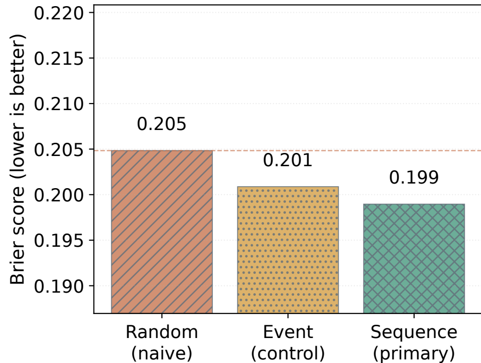
(a) Brier difference: sequence – random = -0.0059
