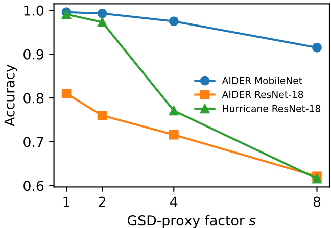
Trust collapse: accuracy vs resolution
