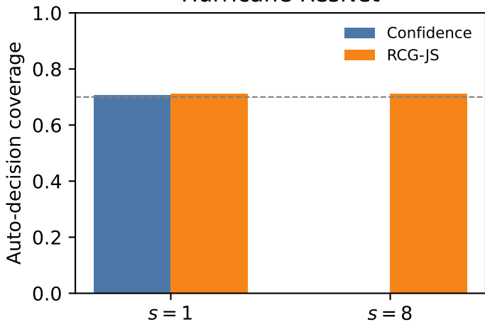
Hurricane ResNet
