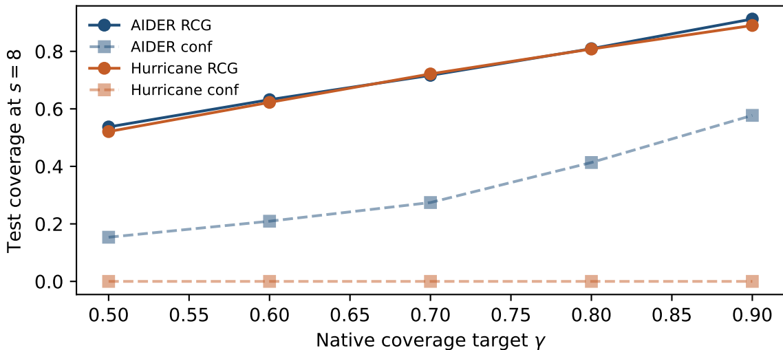
Threshold-transfer coverage across \gamma
