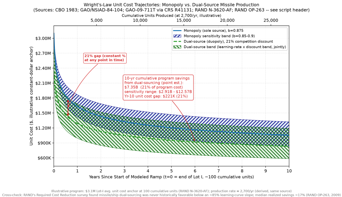
Figure 5: Dual-sourcing's modeled price advantage over a monopoly baseline reaches a point estimate of 21 percent of unit cost by year 10 of a 27,000-unit missile program, with a sensitivity band of 10–30 percent across the underlying learning-curve and competition-discount ranges.
