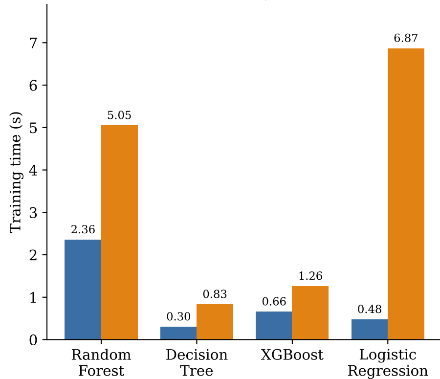
(a) Training time
