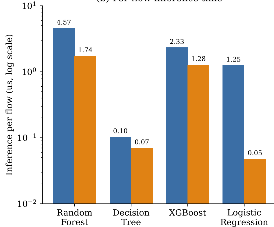
(b) Per-flow inference time
