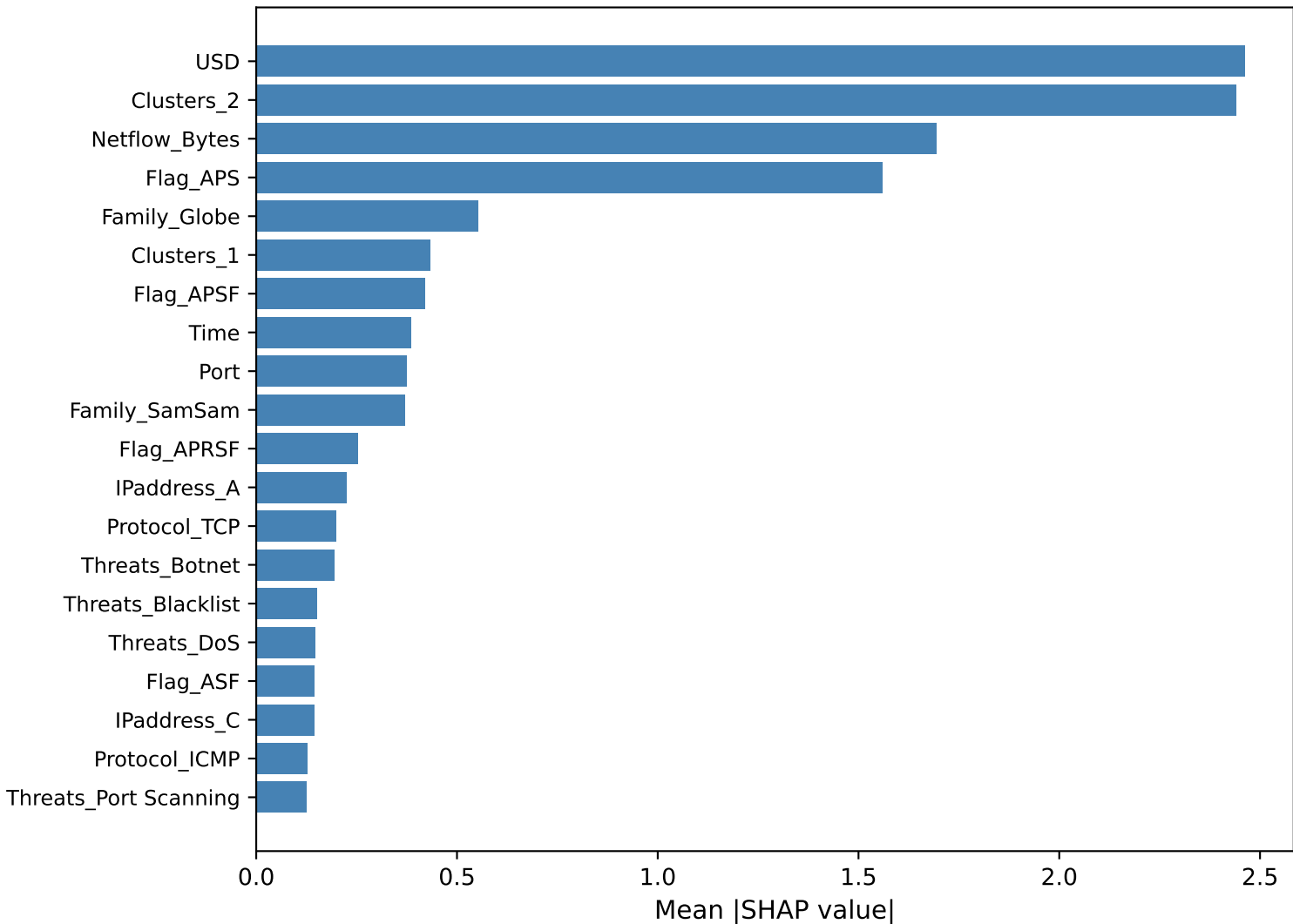
XGBoost Feature Importance (SHAP) - UGRansome2024
