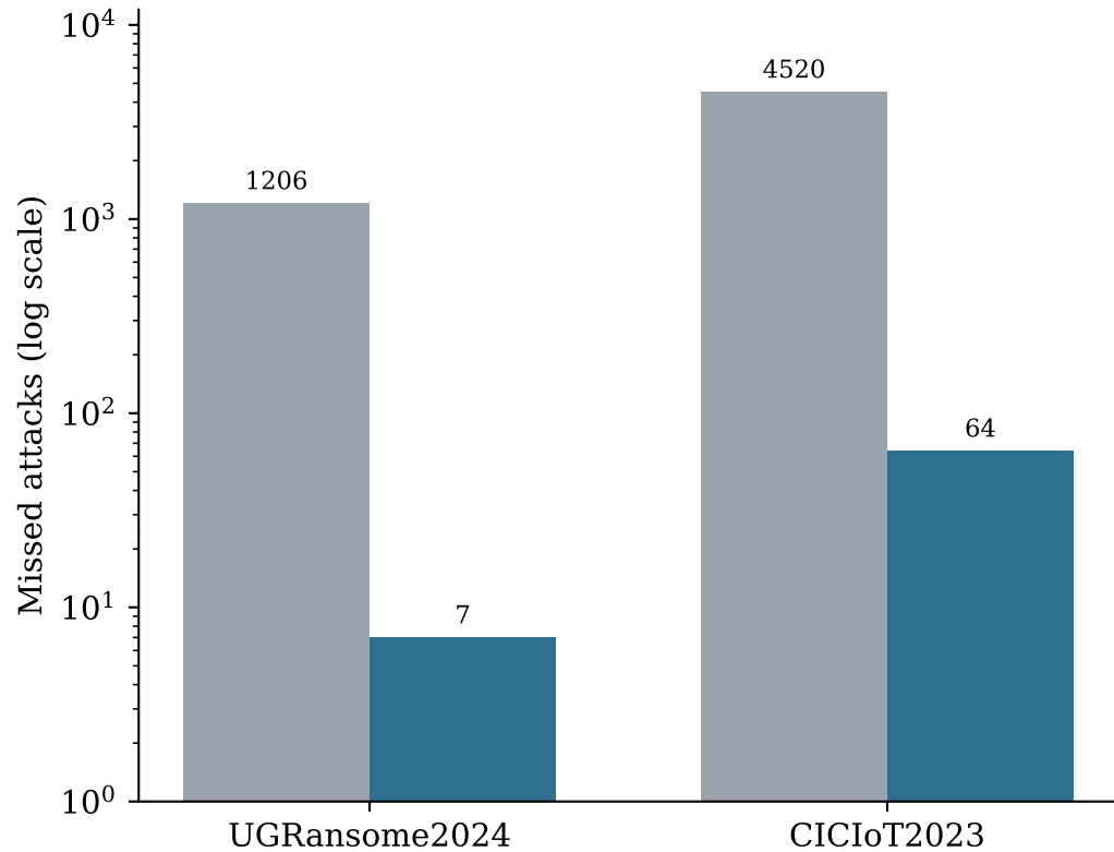
(b) Missed attacks (false negatives)
